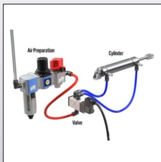
Pneumatic System
